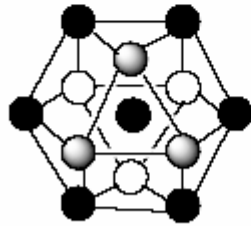
kuboktahedron
