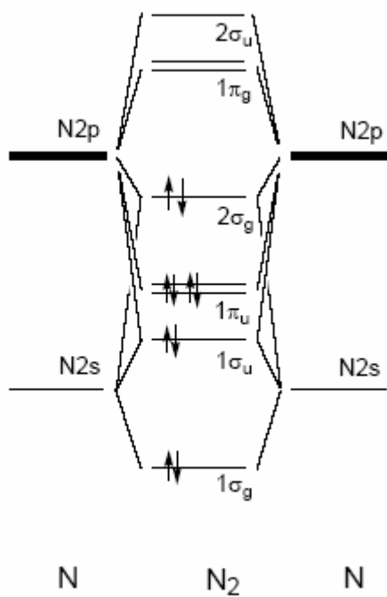
Gambar 2.19 Orbital molekul N 2 .
