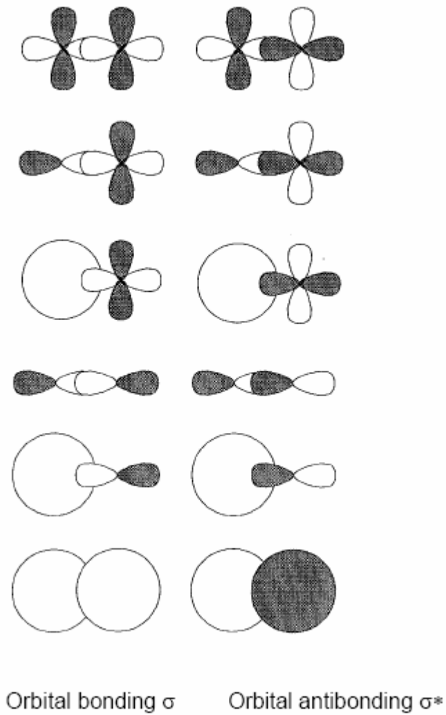
Gambar 2.16 Orbital molekul \sigma .
